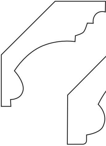
CR-1140 3 1/2" - 2 1/2" drop
